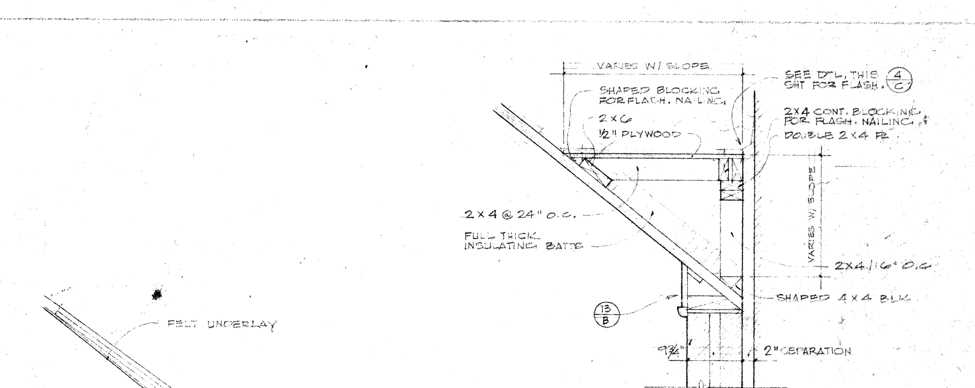
D DORMER VENTS (8 OF THESE) SCALE: HALF SIZE
