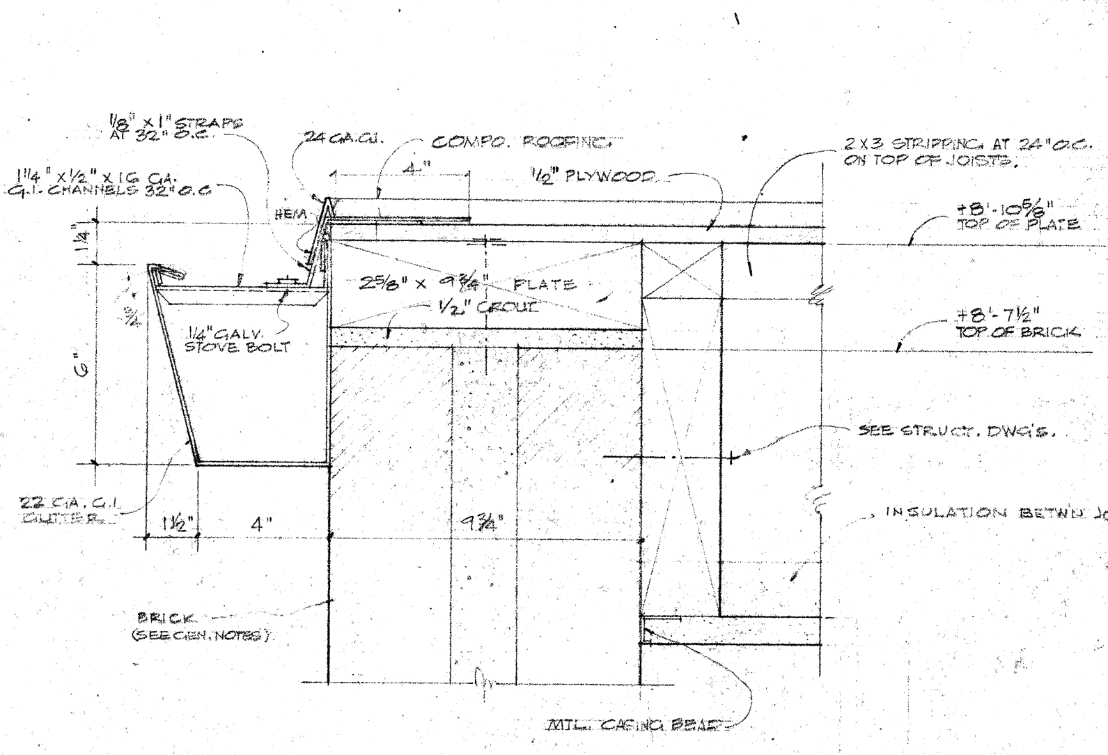
A FLASHING AT FLAT ROOF AT EAST WALL OF AUDITORIUM
