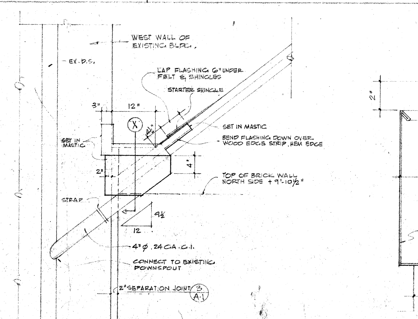
F FLASHING AT INTERSECTION OF SADDLE & PITCHED ROOF SCALE: HALF SIZE
